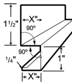
LG 120 DENVER EAVE TRIM
